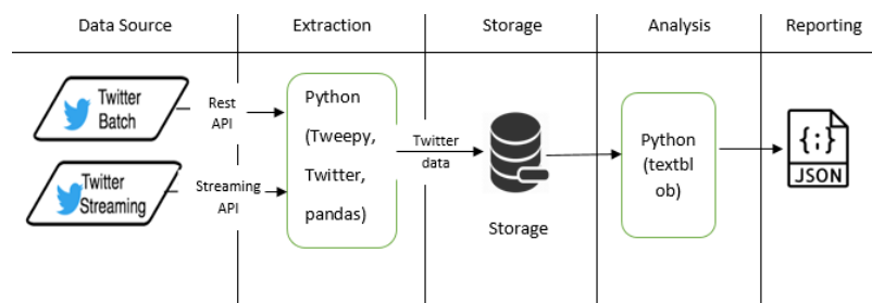
Fig.5. The Architecture of Data Collection.
