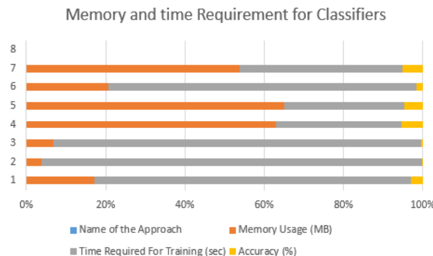
Fig.11. Comparison Between Accuracy, Memory and Time.
